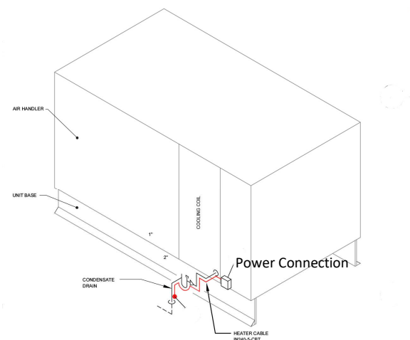
AIR HANDLING UNIT, CONDENSATE DRAIN & HEATER CABLE
